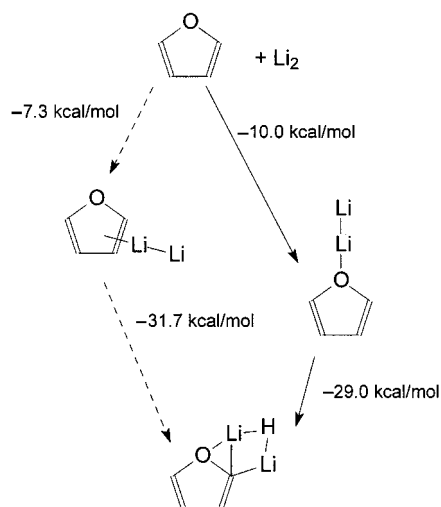
Figure 2. Calculated reaction mechanism for the cocondensation of lithium atoms with furan
