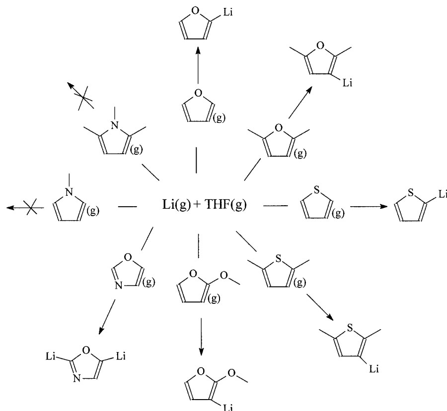
Scheme 5. Summary of the reactions of lithium atoms with five-membered heterocycles in the presence of THF at 77 K
