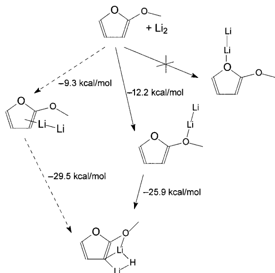
Figure 7. Calculated reaction mechanism for the cocondensation of lithium atoms with 2-methoxyfuran
