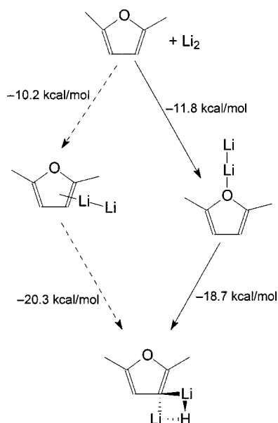
Figure 3. Calculated reaction mechanism for the cocondensation of lithium atoms with 2,5-dimethylfuran
