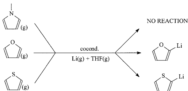
Scheme 1. Cocondensation reaction of lithium atoms with heterocycles at 77 K
