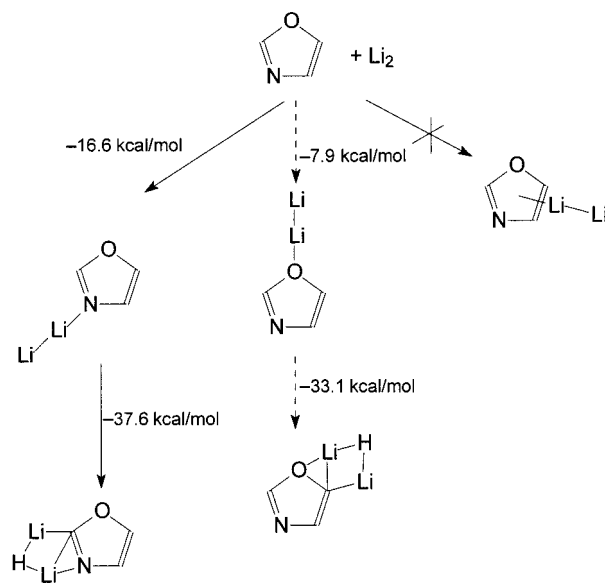
Figure 8. Calculated reaction mechanism for the first lithiation of oxazole
