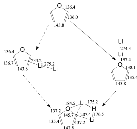
Scheme 7. Bond lengths in pm for furan reaction intermediates
