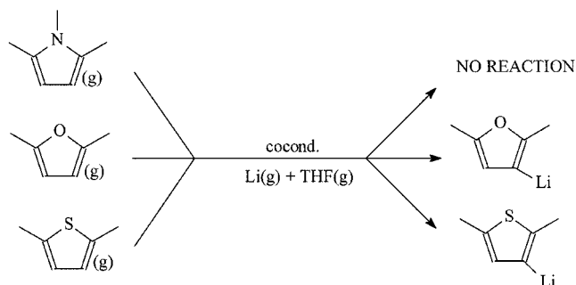
Scheme 2. Cocondensation reaction of lithium atoms with ortho -dimethyl heterocycles at 77 K
