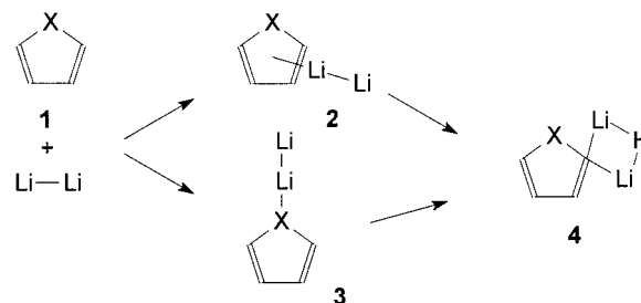
Scheme 6. Key mechanistic steps in heteroaromatic C–H bond activation using lithium atoms
