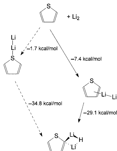
Figure 4. Calculated reaction mechanism for the cocondensation of lithium atoms with thiophene
