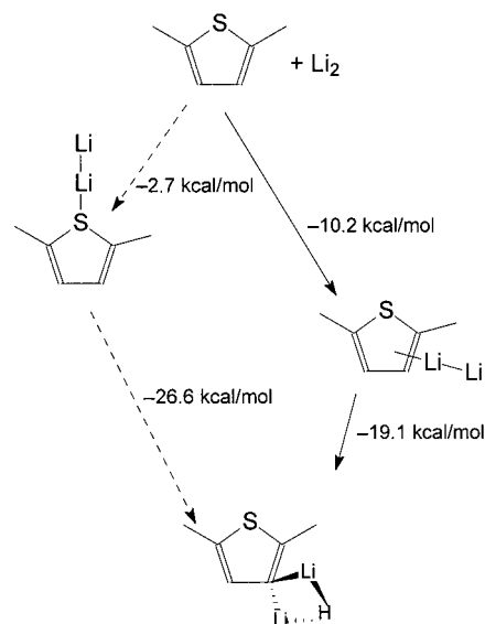
Figure 6. Calculated reaction mechanism for the cocondensation of lithium atoms with 2,5-dimethylthiophene
